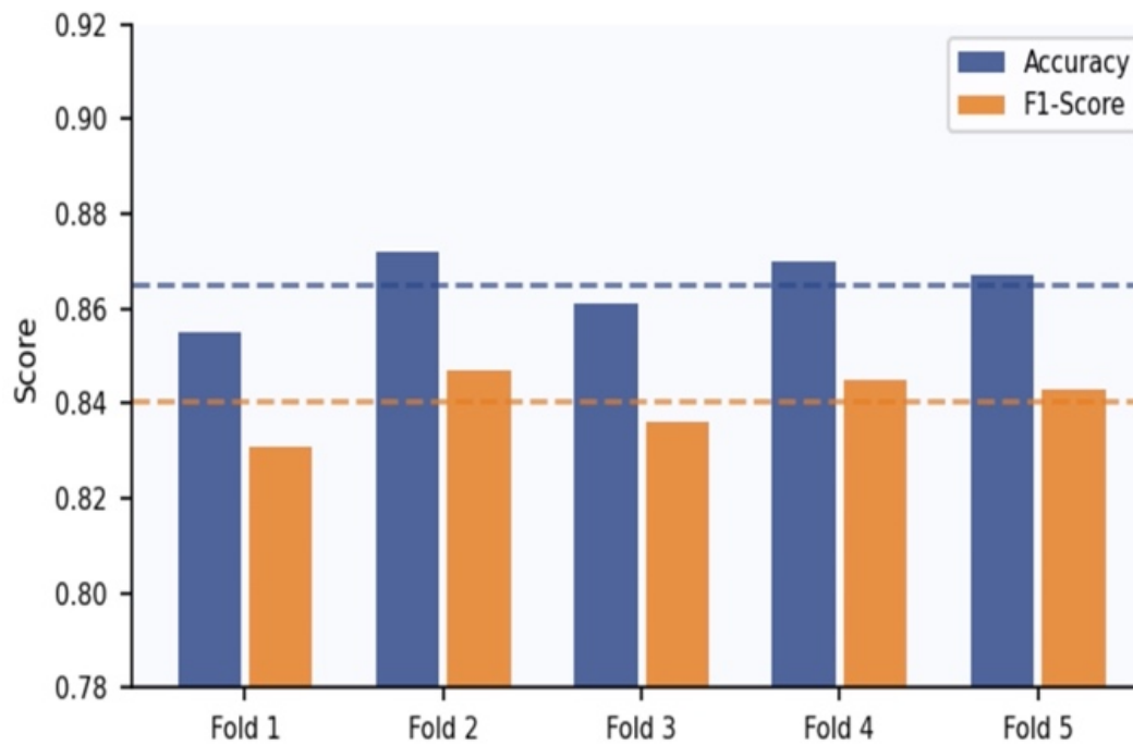
Fig. 9. Five fold Cross Validation Result
